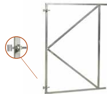
Verstelbaar poortframe - verzinkt 100x80 cm - 2 ogen €66,91 p/st 90x155 cm - 2 ogen €82,30 p/st 100x155 cm - 2 ogen €86,06 p/st 110x155 cm - 2 ogen €92,61 p/st 120x155 cm - 3 ogen €96,73 p/st 130x155 cm - 3 ogen €103,26 p/st 140x155 cm - 3 ogen €108,54 p/st 150x155 cm - 3 ogen €115,99 p/st
